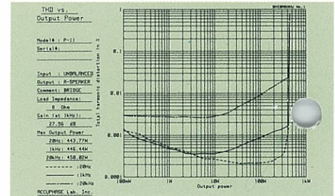
● P-11 Power output vs. THD (8-ohm load, mono operation)
