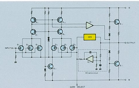
Fig. 2 Equalizer Amplifier Section
